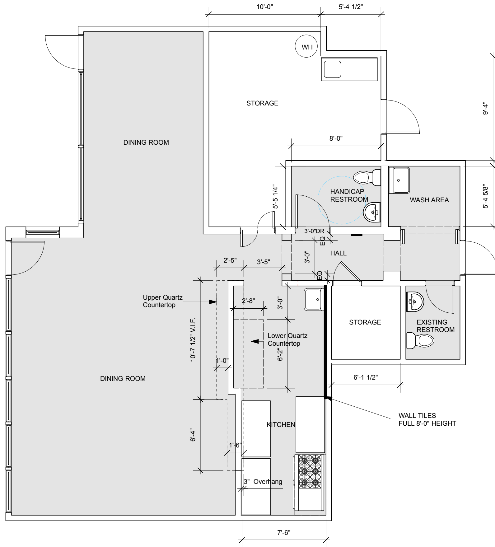
Floor Plan 3/16" = 1'-0"
